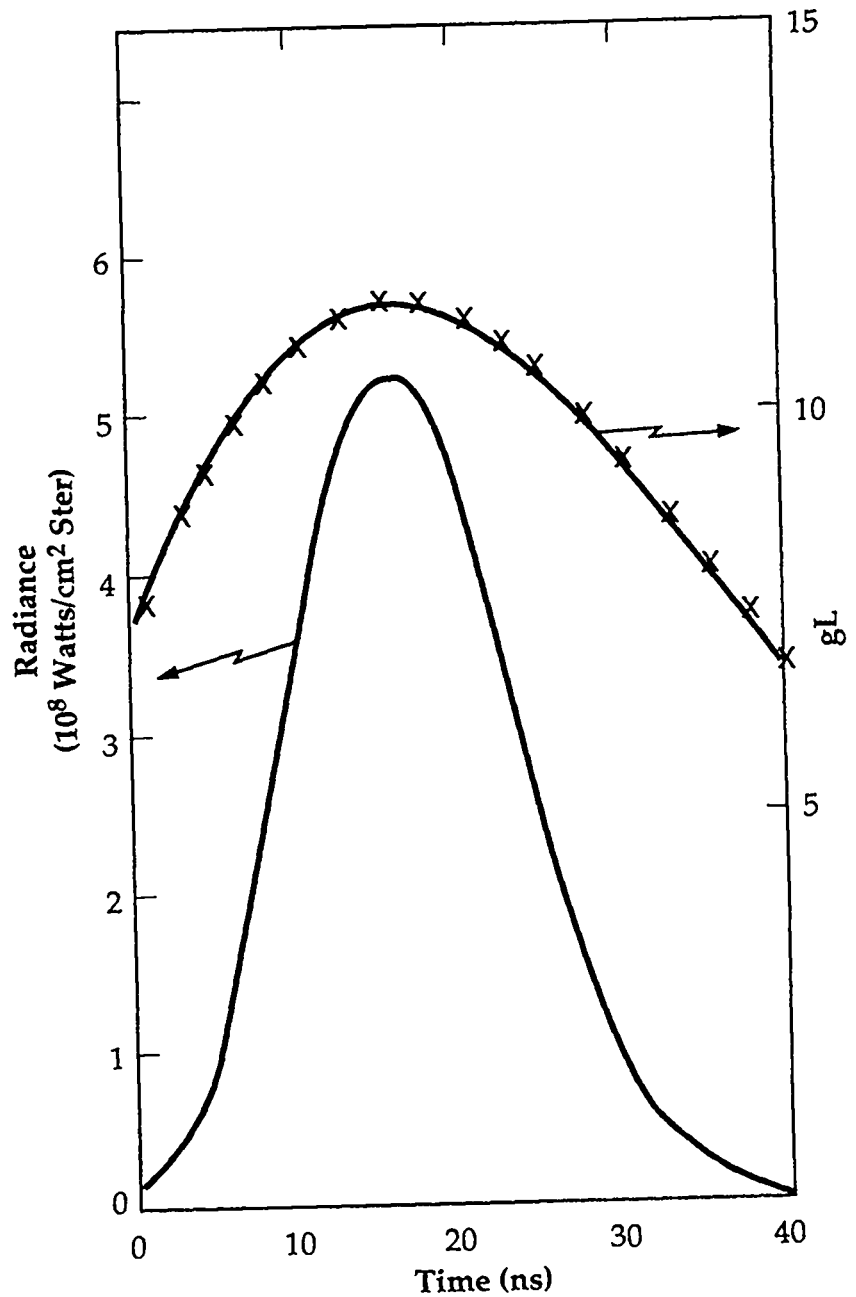
Fig. 3. Measured radiance from Lumonics amplifier and calculated gl.
