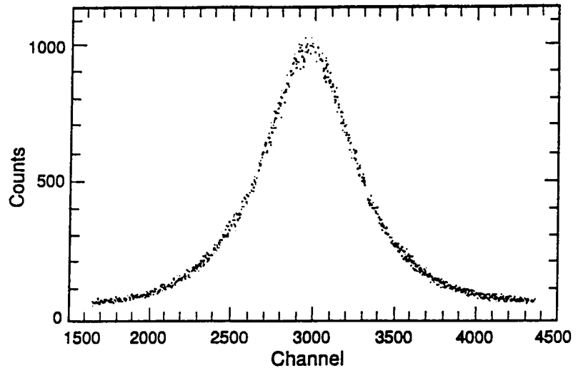
Fig. 5. Transit time spectrum obtained with the two photomultiplier tube method using XP1911 tubes and a BC418 scintillator. The calibration factor is 155 channels per ns. The full width at half maximum corresponds to 4.5 ns.
