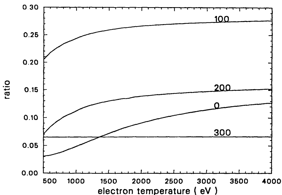
Fig. 5. The 3-1/2-1 line ratio of He-like iron as a function of electron temperature for various radiation temperatures at N_e = 10^{19} \text{ cm}^{-3} . Each curve is labeled by the radiation temperature in eV.
